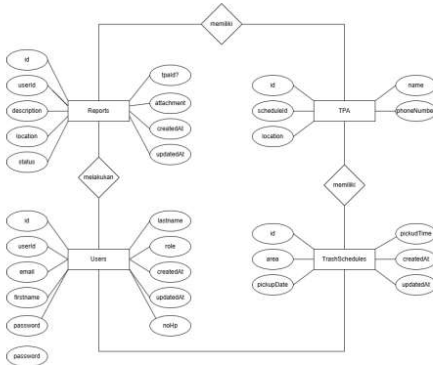
Gambar 2. Entity Relationship Diagram
