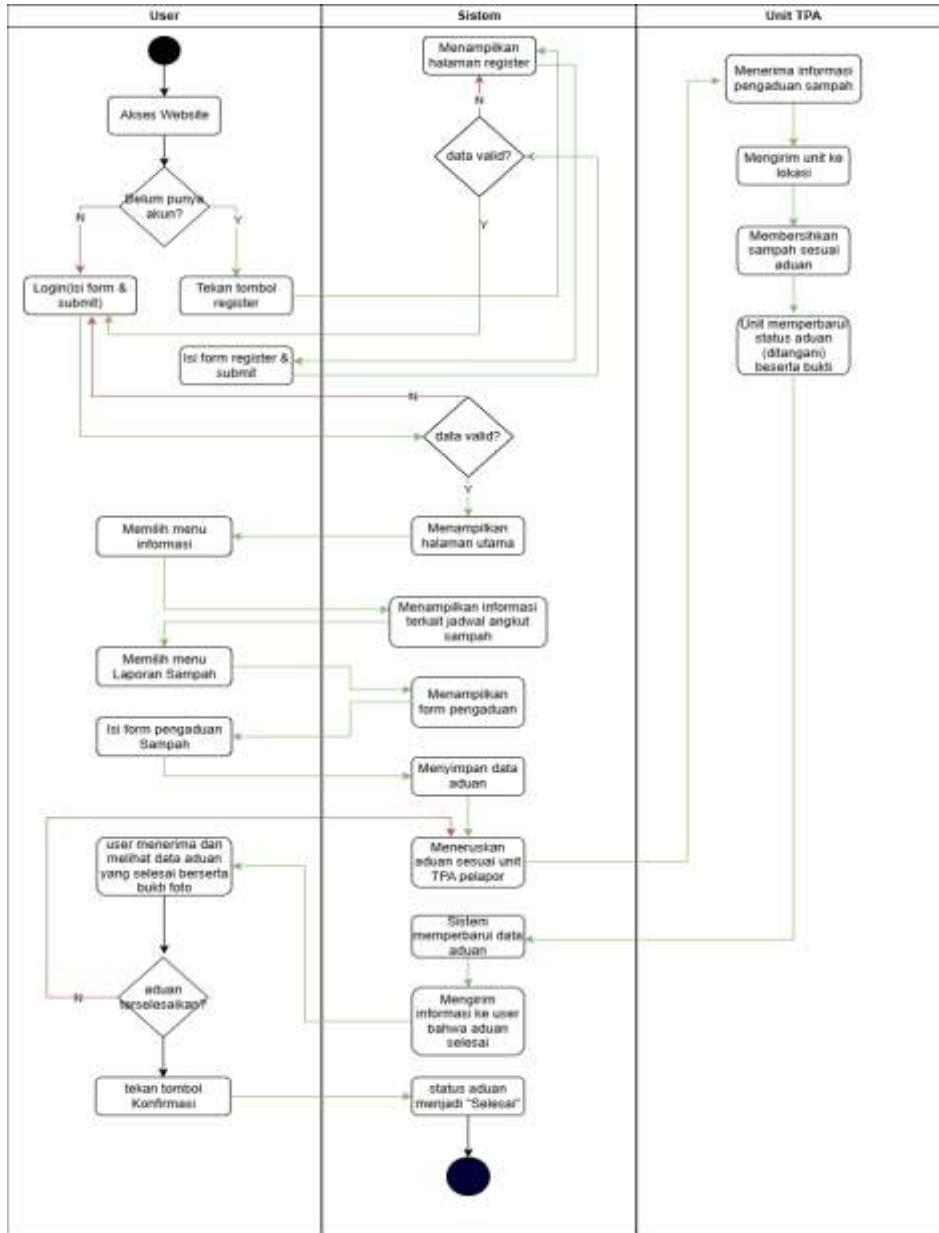
Gambar 1. Activity Diagram System Usulan
